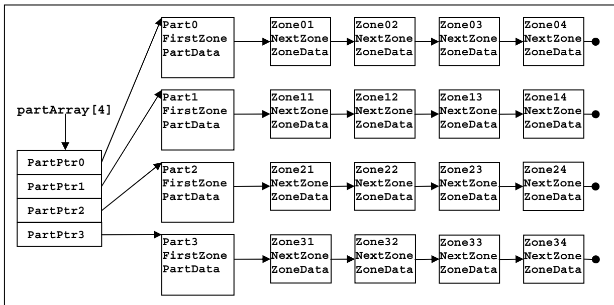
Figure 2 CLOMP unstructured mesh data structures for numParts = 4 and zonesPerPart=4.
